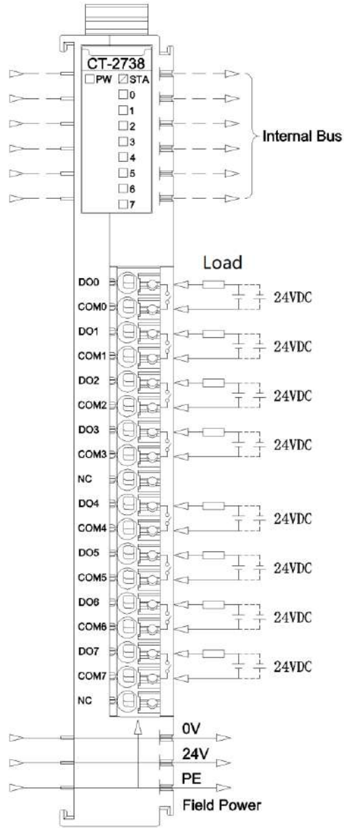
Figure 1 Resistive load wiring diagram
