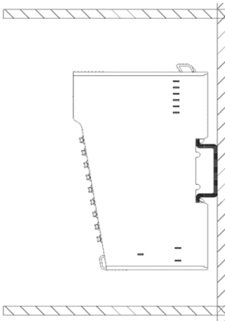
①Right view of vertical installation
